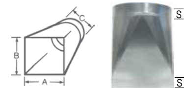
Trans 1 - Square to Round
